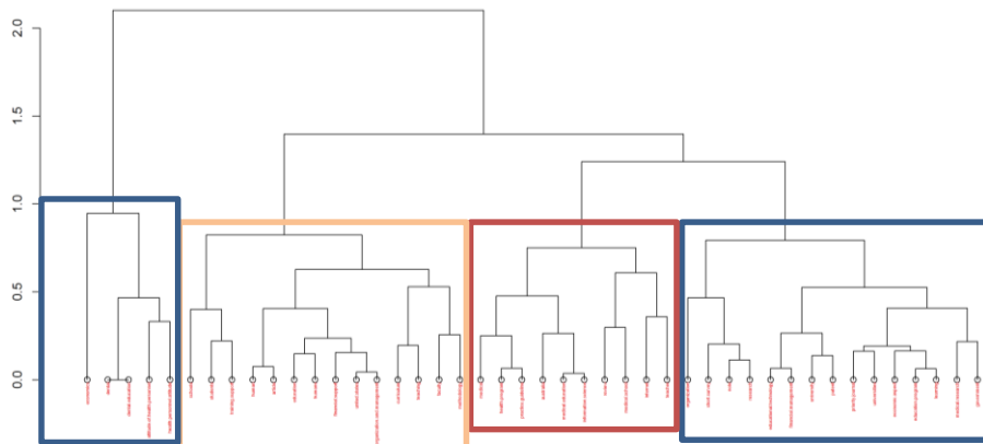
Figure 4. dendrogram results
